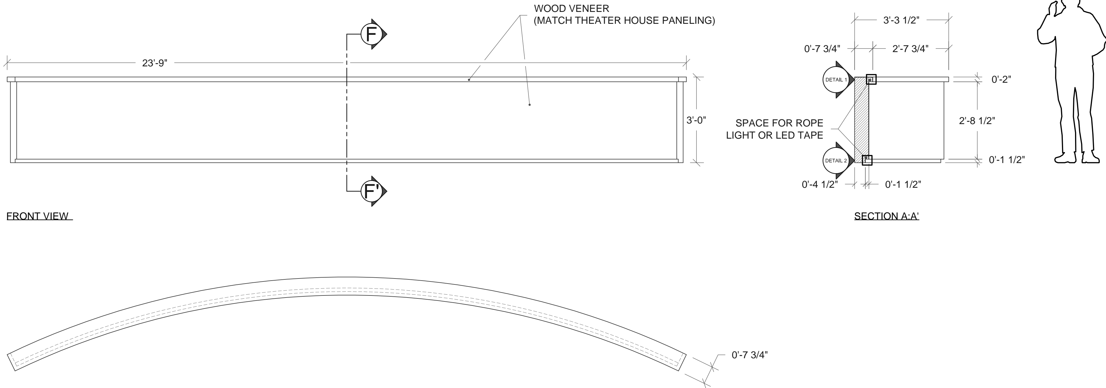
PLAN VIEW
