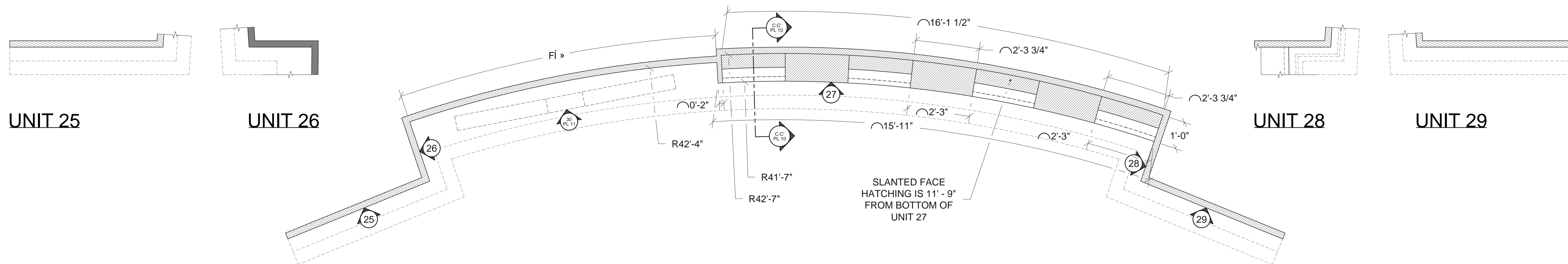
CROSS AND TRINITY WALL LAYOUT
